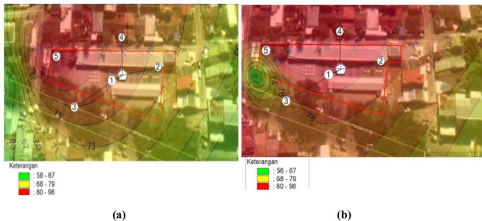
Figure 3. Contour noise level distribution no music and live music in areopala food city.
