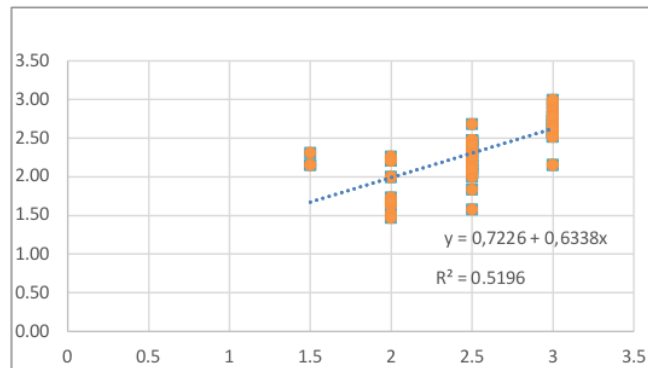
Figure 4. Equation of the regression model equation.
